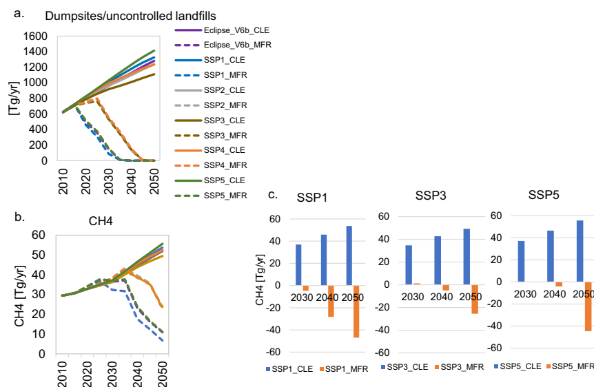
Fig. 4 Global methane emissions under baseline and mitigation scenarios. a Municipal solid waste (MSW) in dumpsites, b Methane ( \text{CH}_4 ) emissions and c \text{CH}_4 reduction potentials (negative values in y-axis in panel c refer to avoided emissions). Faster adoption of measures improving MSW systems will result in an early decrease of MSW ending up in dumpsites/uncontrolled landfills and therefore brings quicker reductions of future \text{CH}_4 emissions from this source. Supplementary Information section 2 presents a detailed analysis of the mitigation (MFR) scenarios.
